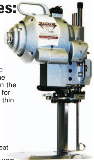
Model 818-8" Straight-Knife Cloth-Cutting Machine
