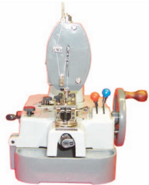
End View of CM491
